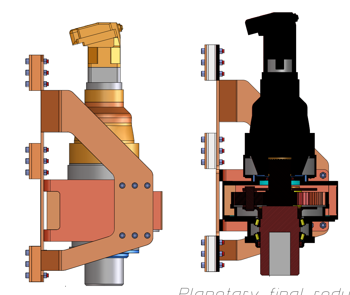
Planetary final reduction
